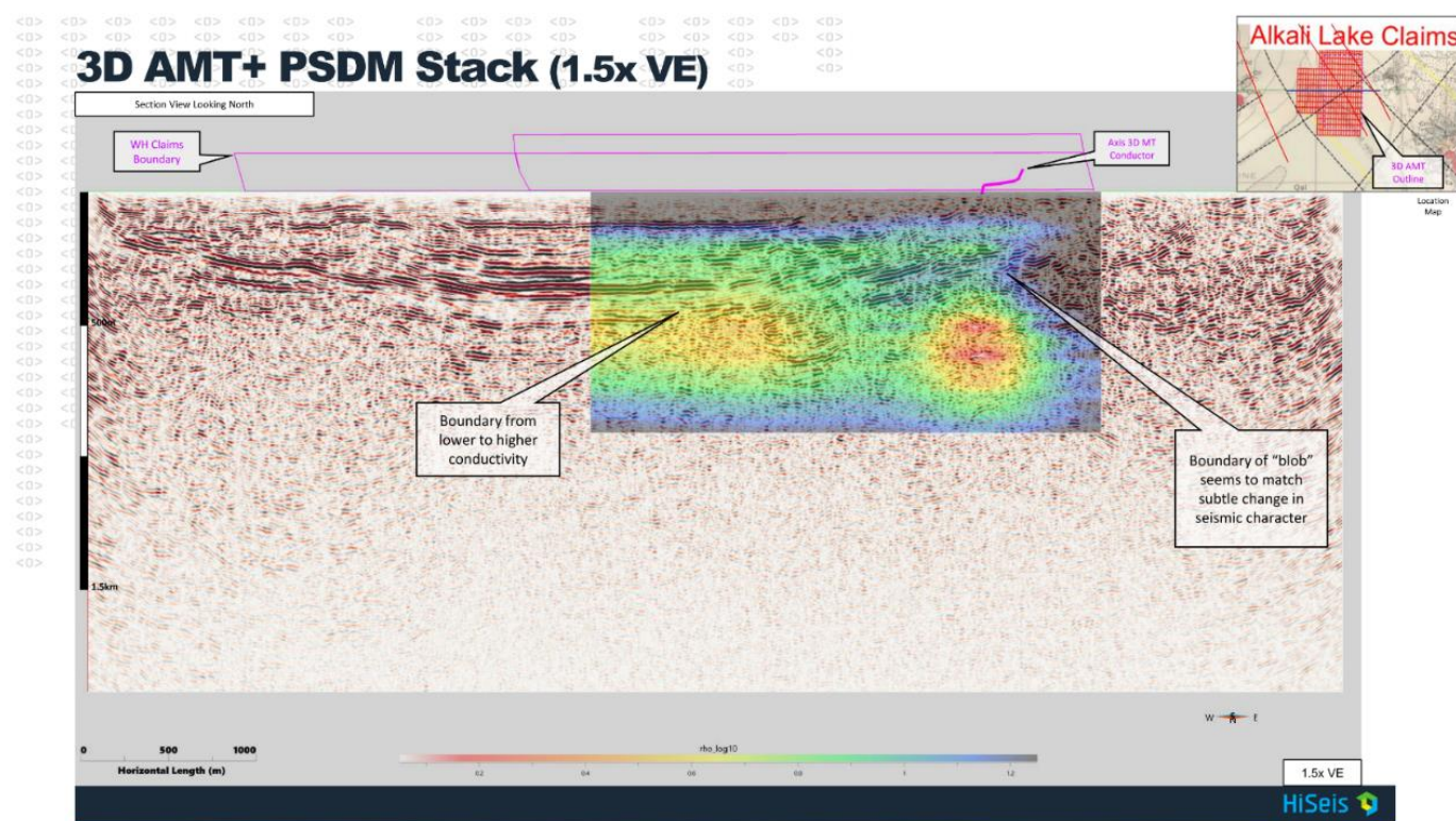
Figure 1. 2D Shallow Seismic Survey results superimposed on 3D AMT Survey Results (refer ASX Release 14/10/2021 )
